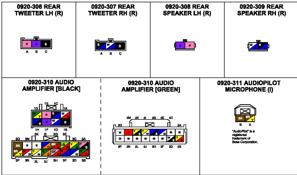
Connectors 0920-3c
