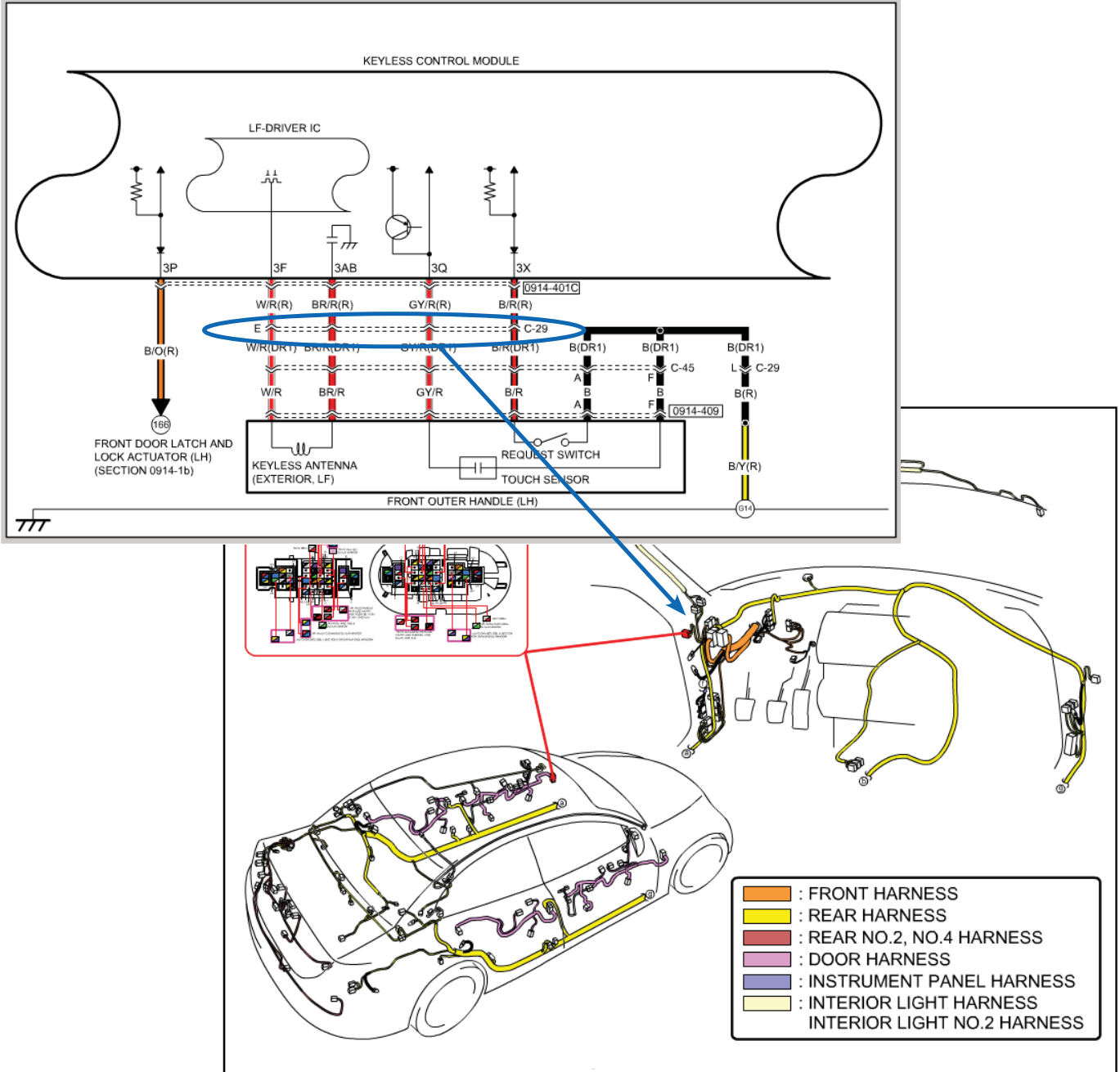
ADVANCED KEYLESS ENTRY AND PUSH BUTTON START SYSTEM (INCLUDES TPMS INFORMATION) 0914-4g
