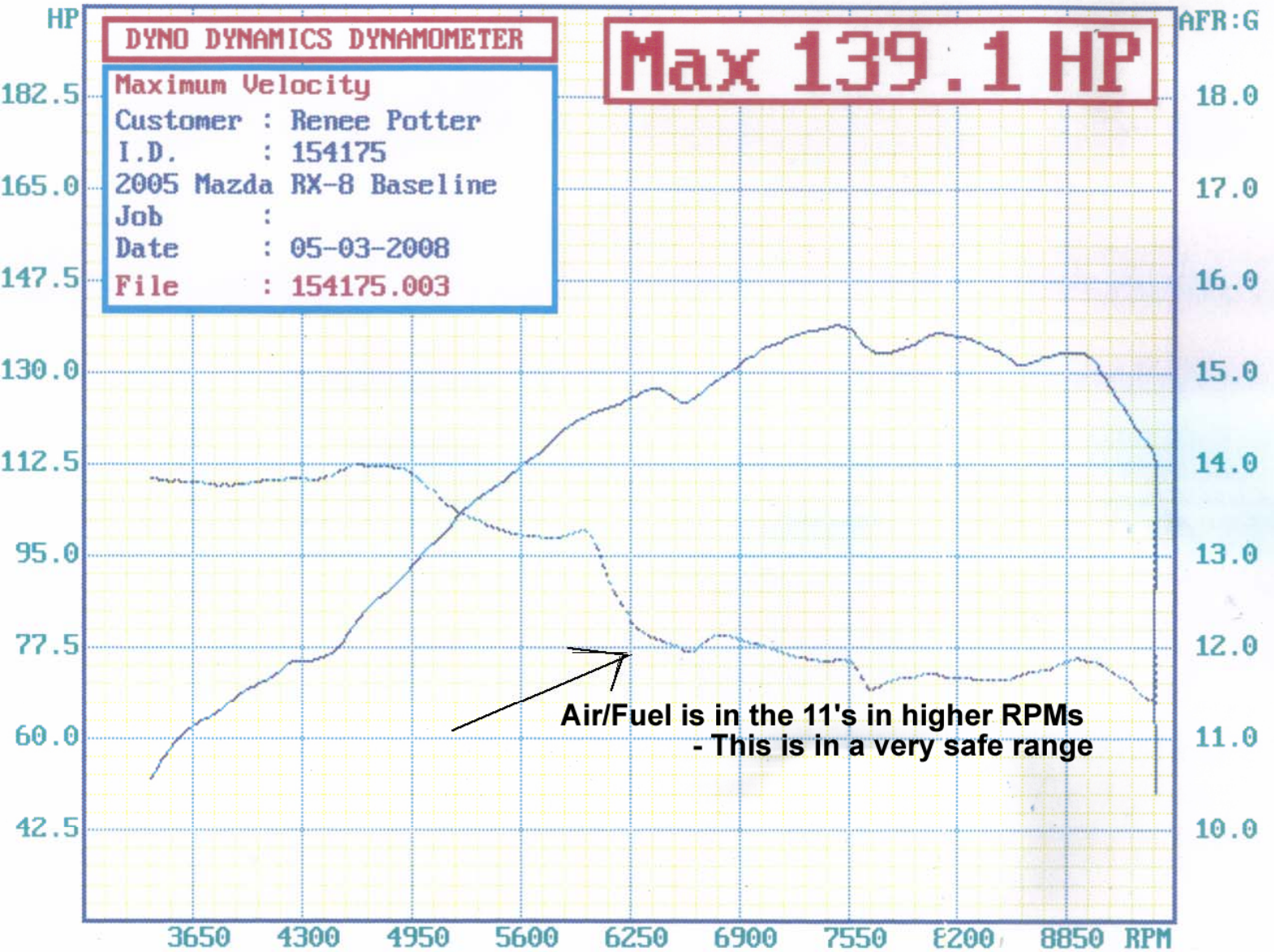
Horsepower and Air/Fuel Ratio graph (Air/fuel is read on the right side)
