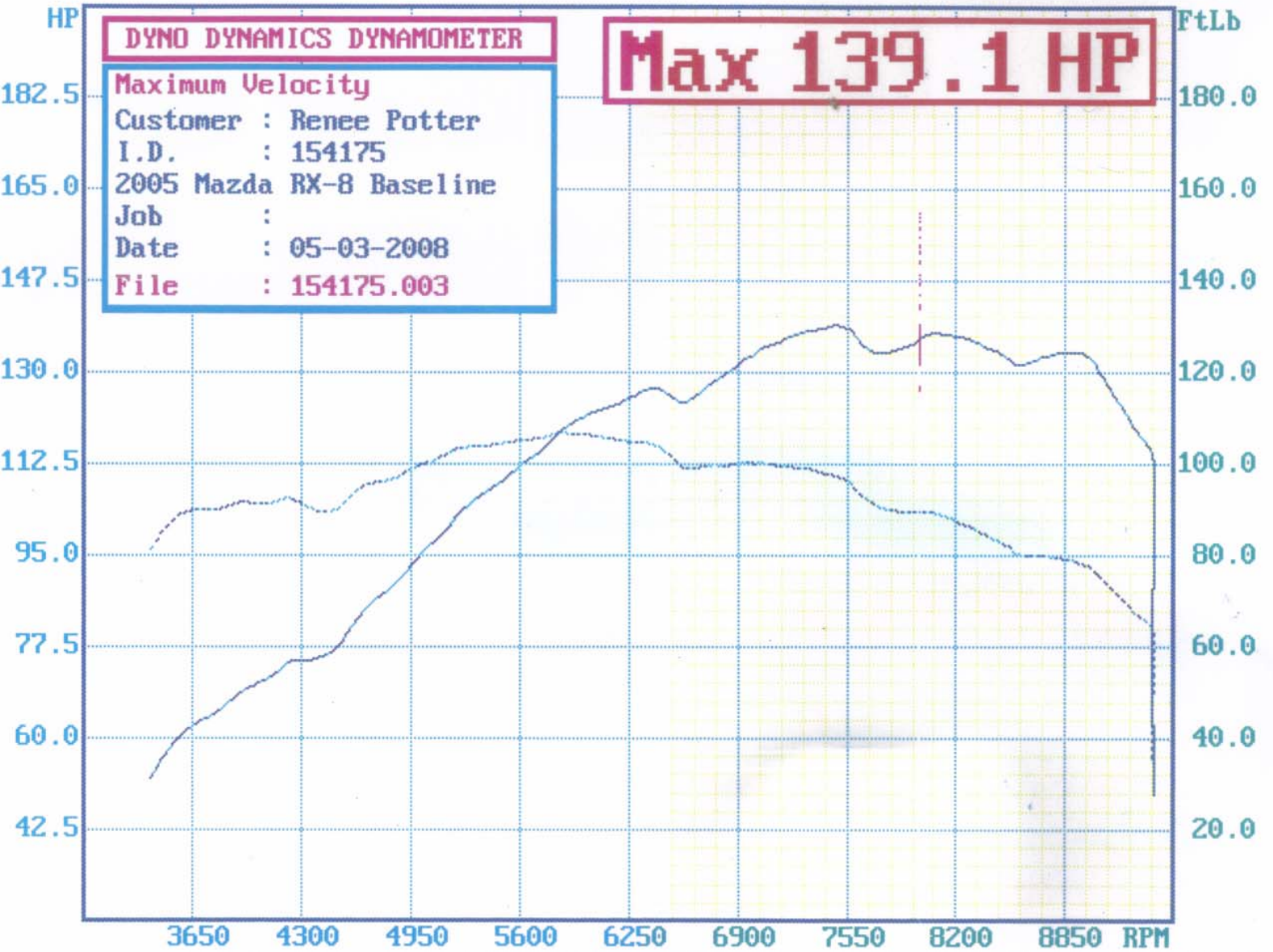
Horsepower & torque graph - Dotted line is torque, (right side axis)
