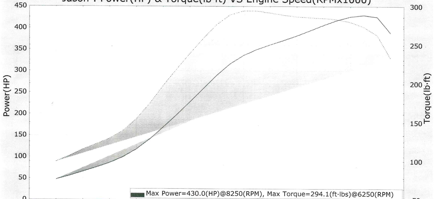
Jason : Power(HP) & Torque(lb-ft) VS Engine Speed(RPMx1000)
