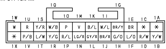
J2-07 AUDIOPILLOT MICROPHONE (I)
