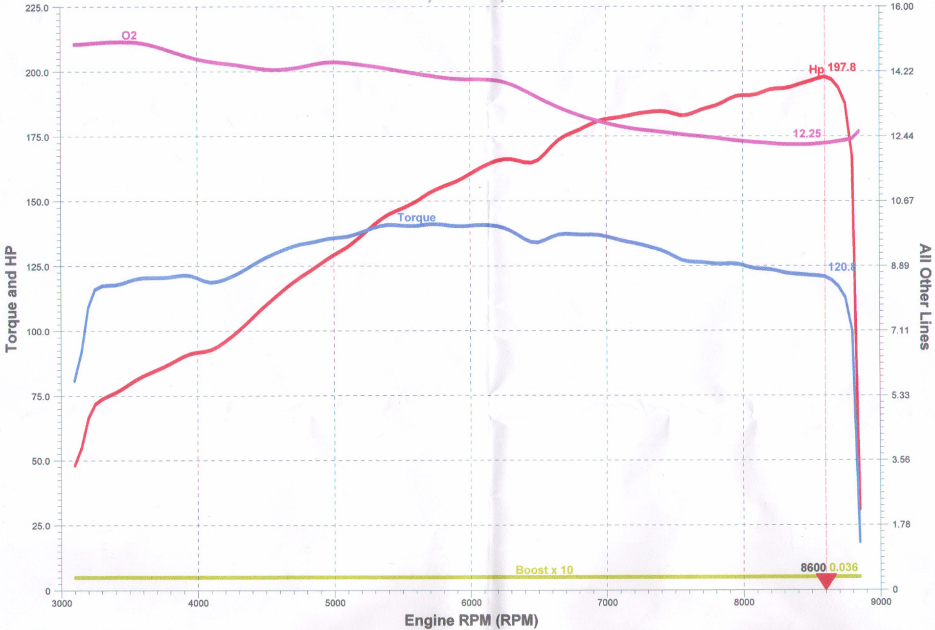
Peak Torque* and Hp* vs. RPM
