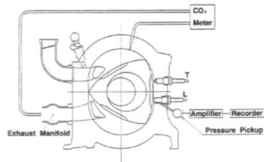
Fig. 12 Test Equipment
