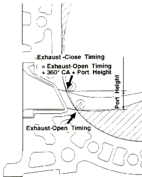
Fig. 5 Geometric Relation Between Exhaust Open and Closure Timings of the Peripheral Exhaust Port RE
